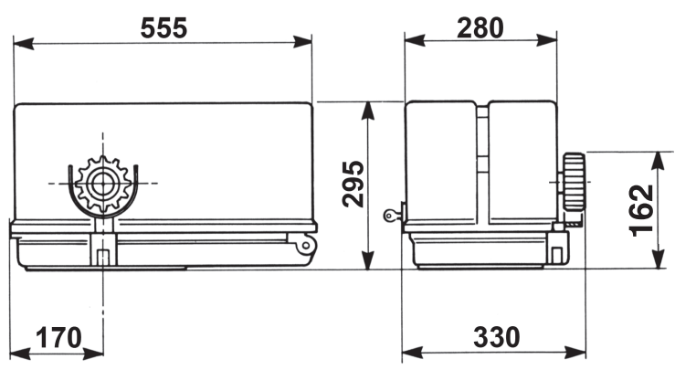
Abmessungen in mm
